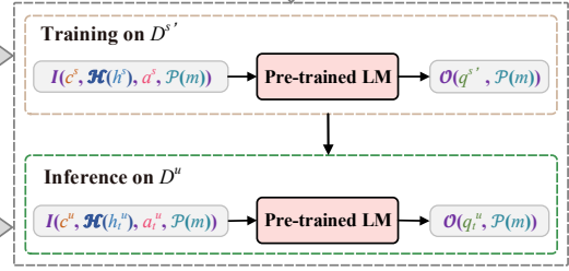
Figure 1: Illustration of the proposed SPARTA for ZeroCQG. (1) Synthesize. For each single-turn QG instance (c^s, a^s, q^s) \in D^s , the conversation synthesis module will retrieve t - 1 question-answer pairs from D^s as simulated history h^s , and transform the q^s into q^{s'} if there exist co-reference with pronoun, e.g. Beyoncé and she . We term the dataset with synthesized conversation as D^{s'} = \{(c^s, h^s, a^s, q^{s'})\} . (2) Prompt. We propose conversation prompting to reformulate the input and output of conversational QG. (3) Transfer. We fine-tune pre-trained LM on the prompted D^{s'} . Then, the fine-tuned pre-trained LM with the same conversation prompting is directly applied for inference on D^u to generate conversational questions.
