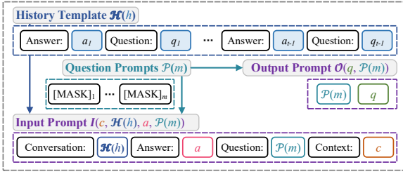
Figure 1: Illustration of the proposed SPARTA for ZeroCQG. (1) Synthesize. For each single-turn QG instance (c^s, a^s, q^s) \in D^s , the conversation synthesis module will retrieve t - 1 question-answer pairs from D^s as simulated history h^s , and transform the q^s into q^{s'} if there exist co-reference with pronoun, e.g. Beyoncé and she . We term the dataset with synthesized conversation as D^{s'} = \{(c^s, h^s, a^s, q^{s'})\} . (2) Prompt. We propose conversation prompting to reformulate the input and output of conversational QG. (3) Transfer. We fine-tune pre-trained LM on the prompted D^{s'} . Then, the fine-tuned pre-trained LM with the same conversation prompting is directly applied for inference on D^u to generate conversational questions.
